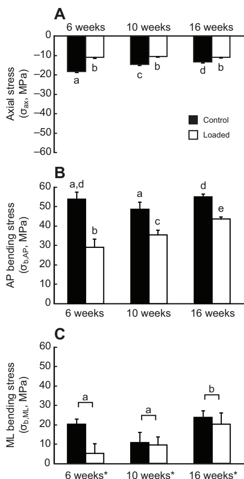
Fig. 7. Stress calculations for the loaded and control tibiae under a 9 N axial compressive load for the 6-, 10- and 16-week-old mice. (A) Axial stress, \sigma_{ax} , (B) anterior-posterior bending stress, \sigma_{b,AP} , and (C) medial-lateral bending stress, \sigma_{b,ML} . Values shown are means \pm 1 s.d. Data for the control and loaded tibiae are shown in black and white, respectively. Different letters above the bars or bracketed pairs of bars indicate significant differences in the means by linear mixed model with repeated measures, followed by pairwise comparisons with Bonferroni correction ( P < 0.05 ). Letters and brackets above the pairs of data bars in C indicate main effect differences with age. Asterisks (*) next to the age group labels in C indicate a main effect difference between the loaded and control limbs across the three age groups corresponding to a general decrease in \sigma_{b,ML} in the loaded tibiae.
